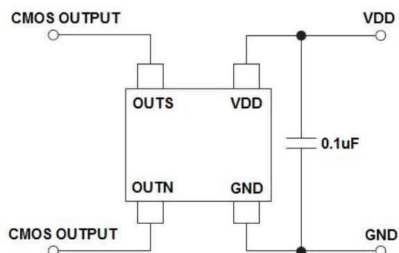
Figure 1, Typical Application Circuit of AS1821S
