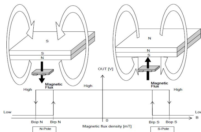
Fig 4, Magnetic Operation Characteristic of AS1821S
