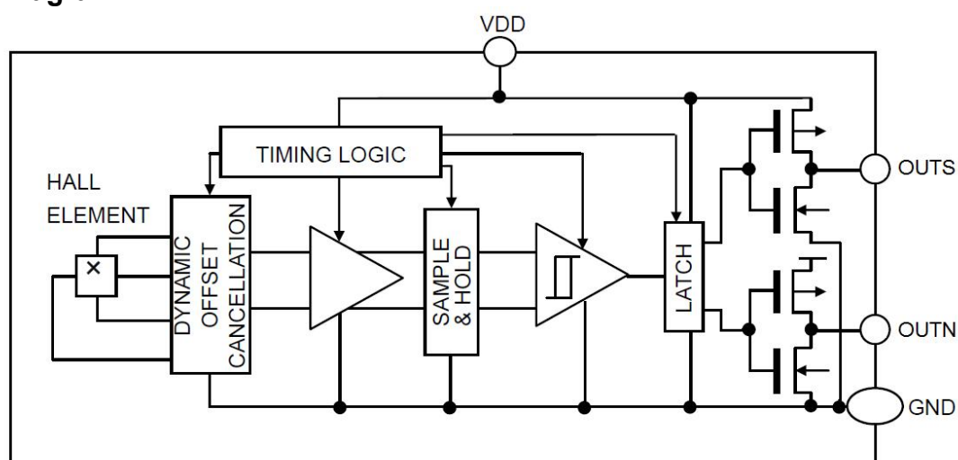
Figure 3, Block Diagram of AS1821S
